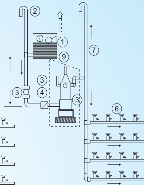
TYPICAL DOWNFEED SYSTEM
