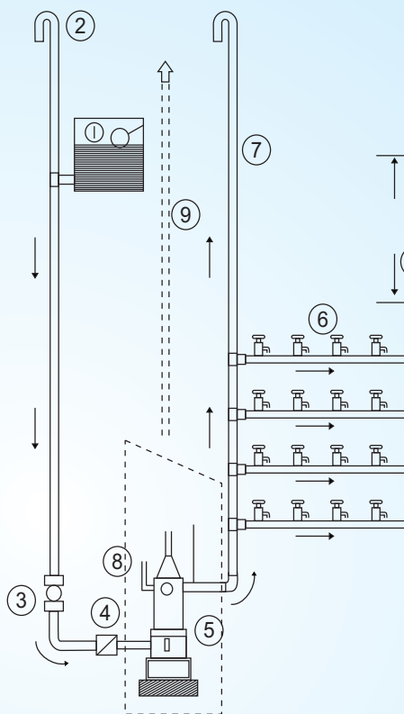
TYPICAL UPFEED SYSTEM
